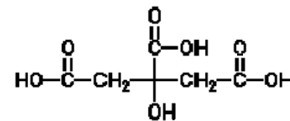
Citric acid
