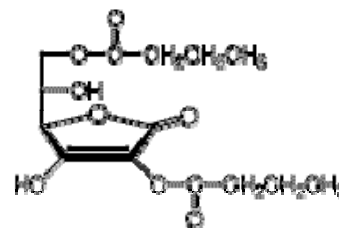
Ascorbic acid
